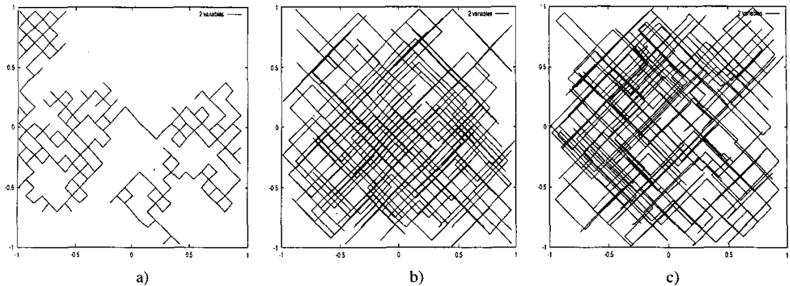
Figure 2: The trajectory of the highest peak's movement over 500 generations in each of the three dynamic environments respectively - a) A = 1.2 ; b) A = 3.3 ; and c) A = 3.99 .
