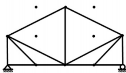
(b) Two-tier, 13-member, 8-node truss
