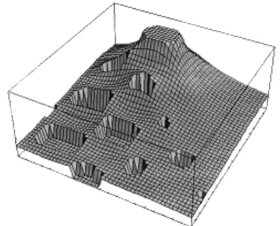
Fig. 16. Levy no. 5 function after the stretching transformation (14).
