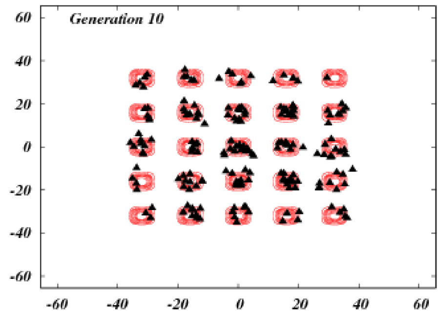
DE/rand/1 population
