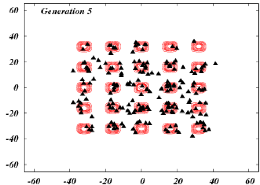
DE/rand/1 population
